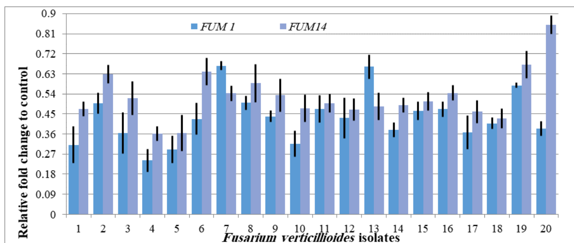
Figure 4. Effect of Bunium persicum essence on transcript levels of FUM1 and FUM14 genes of Fusarium verticillioides isolates. Error bars indicated the standard error of three independent replicates. Data calculated using the \Delta\Delta CT method were expressed as relative units.
